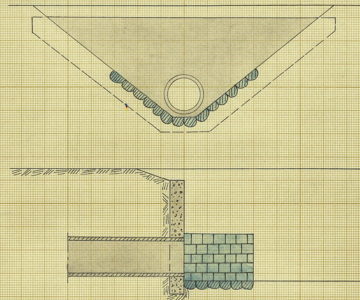
Skala = 1:150
